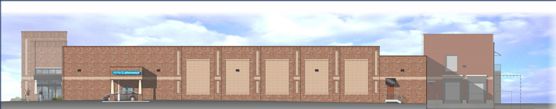
RIGHT SIDE ELEVATION - NORTH (FACING NORTH LOOP ROAD)
